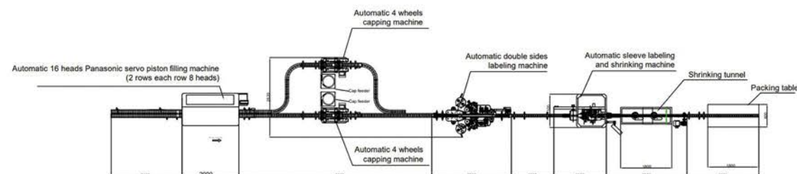
Total length 22.4m, Max width 2.82m, Max height 2.2m
